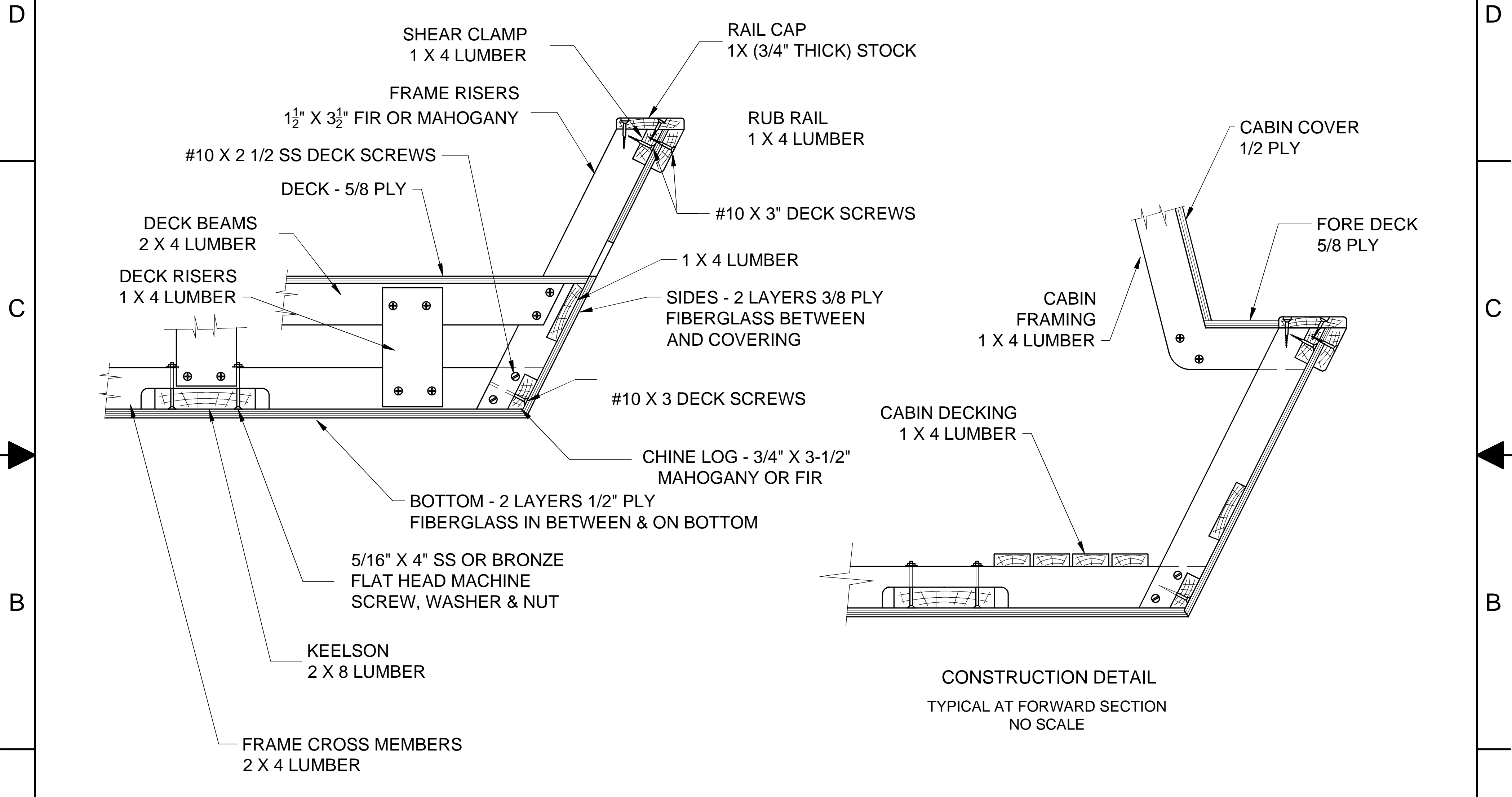
CONSTRUCTION DETAIL TYPICAL AT AFT SECTION NO SCALE
